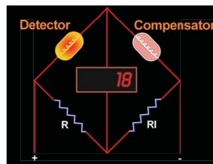
Figure 4: Typical catalytic bead sensor operation
