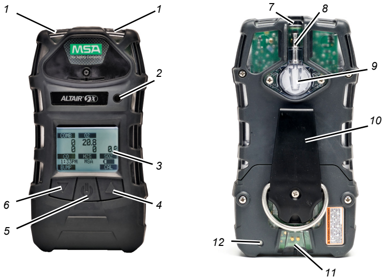
Fig. 1 Device view
